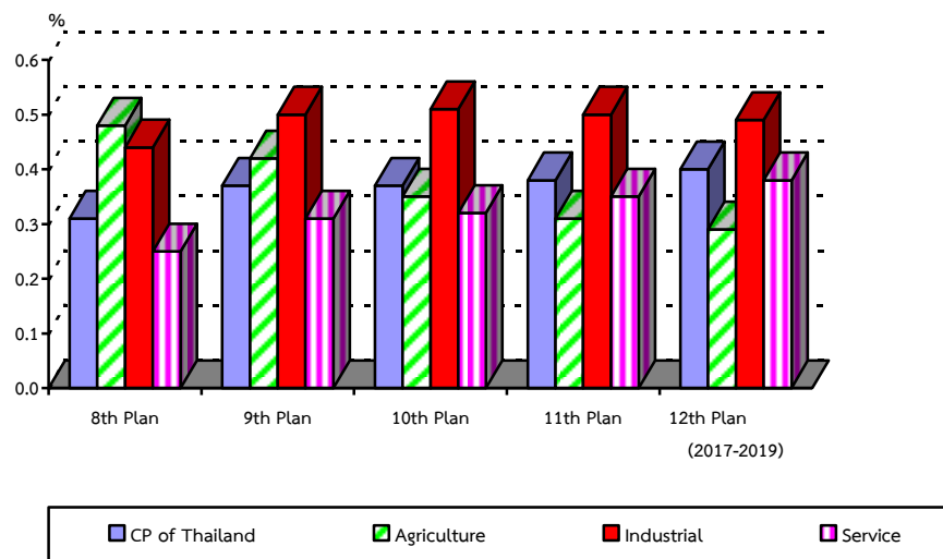
Figure 7 Capital Productivity
